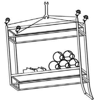
STEP 6 use parts C
